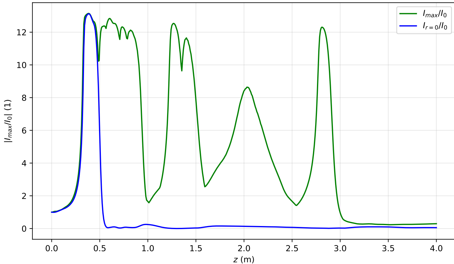
I_{\max}(x=0, y=0, z)/I_0 , P_{\text{in}}=8.5P_{\text{cr}} , noisy input, artificial time
